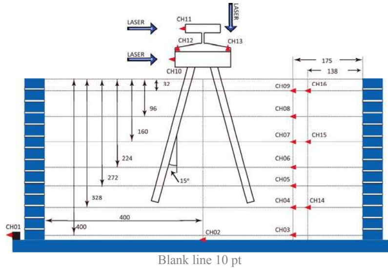
Figure 2.4 Arrangement of accelerometers and laser sensors for the inclined pile group
