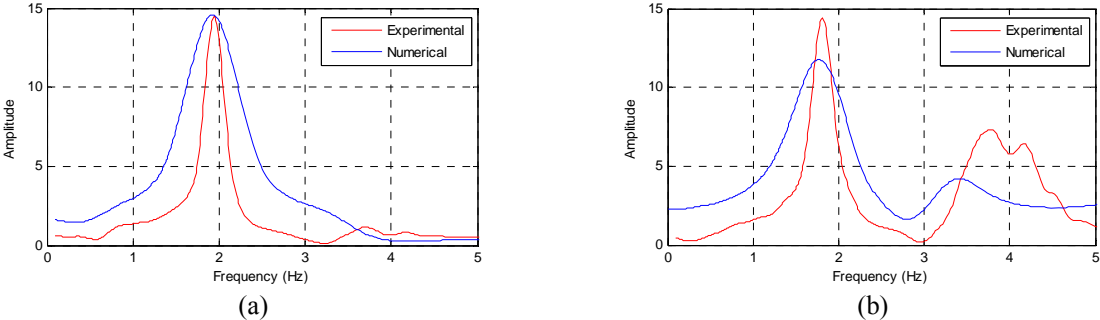
Figure 4.1 Transfer function between the top building output acceleration and the base input signal: (a) inclined pile group (b) vertical pile group
