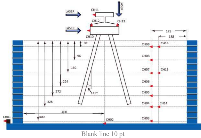
Figure 2.4 Arrangement of accelerometers and laser sensors for the inclined pile group
