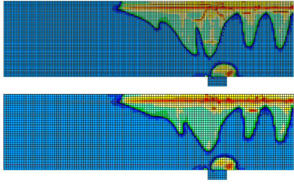
Figure 10.4. F = 1837\text{kN}
