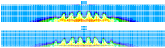
Figure 5.2. 4mm displacement
