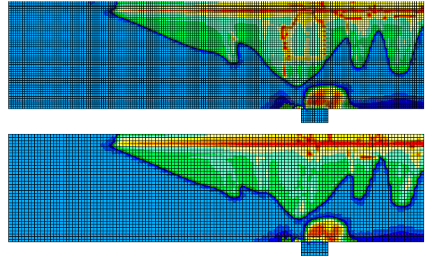
Figure 10.5. F = 2250\text{kN}
