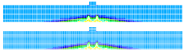
Figure 5.1. 2mm displacement
