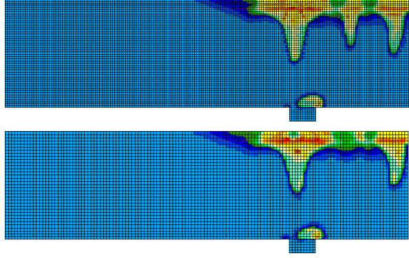
Figure 10.2. F = 1185\text{kN}
