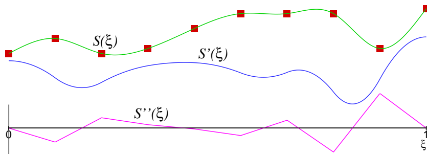
Figure 2: A B-spline interpolation S(\xi) , its first derivative S'(\xi) and its second derivative S''(\xi) with natural end boundary conditions
