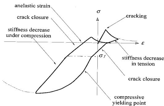
FIGURE 3. Tension-compression cycle
