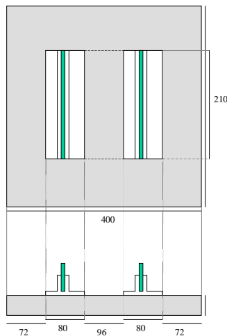
FIGURE 10. Strip foundations and sand container
