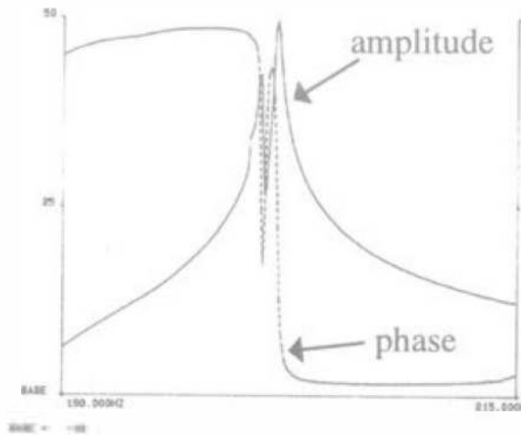
Figure 4. Casing frequency response.
