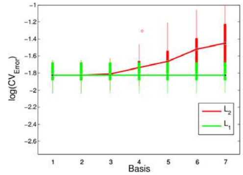
FIGURE 8. Cross validation error of \ell_1 and \ell_2 regularized update for sample size Q = 100
