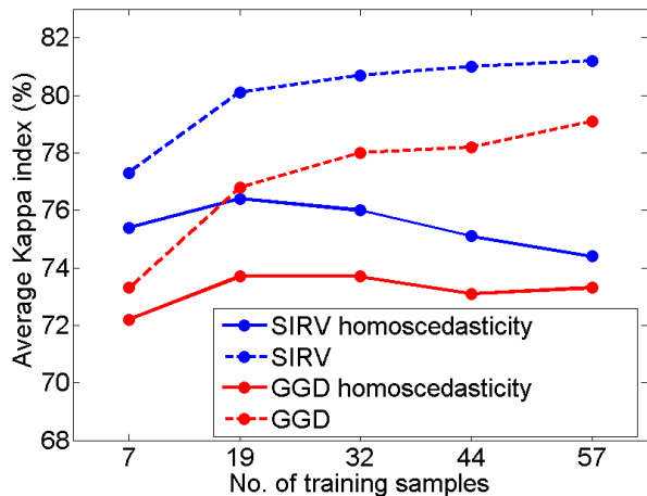
Fig. 2. Evolution of the average kappa index as a function of the number of training samples on the VisTex database for the univariate GGD and the SIRV models.
