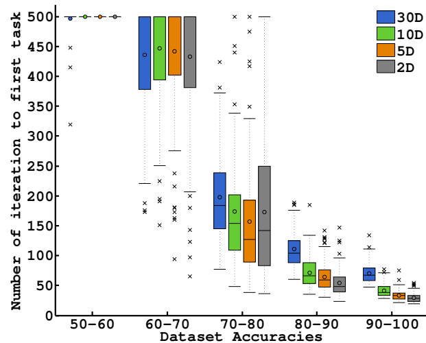
Figure 3: Number of steps to complete first task using artificial data. Under 60 percent accuracy, the confidence threshold cannot be reached in 500 steps. The dataset qualities, more than their dimensionality, impact the learning time.
