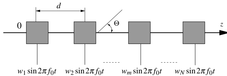
Fig. 1. An uniform antenna array
