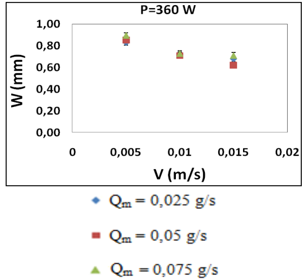
Figure 16. For each laser power, observations of the variation of the width W as a function of velocities V for the three mass flow Q_m .
