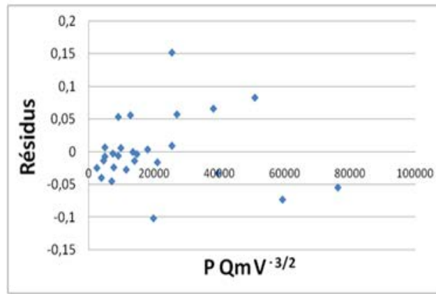
Figure 20. a) Clad area versus PQmV^{-3/2} . b) Residuals.
