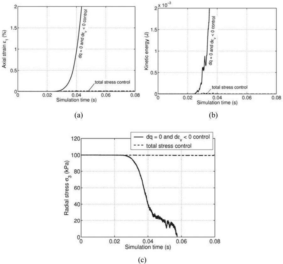
Figure 9.10. Comparison of the responses along a q -constant path simulated with a loose specimen for a full stress control and a control in dq = 0 and d\epsilon_v < 0
