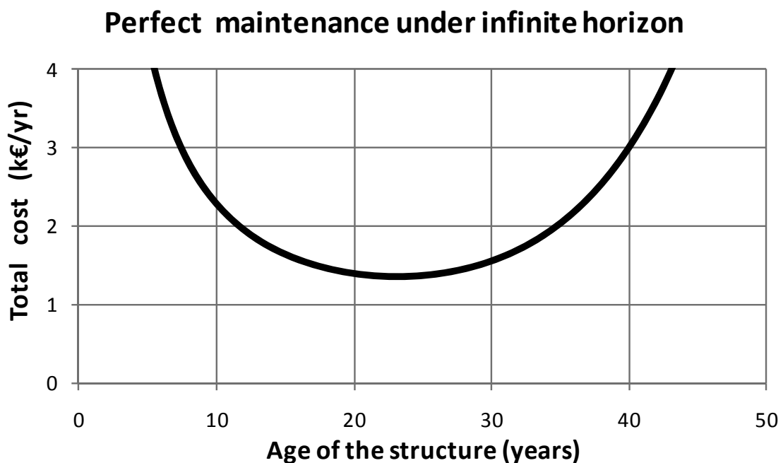
Figure 14.8. Perfect maintenance cost according to time interval between operations
