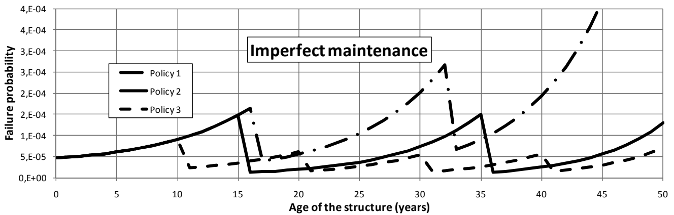
Figure 14.11. Evolution of the failure probability (imperfect maintenance)
