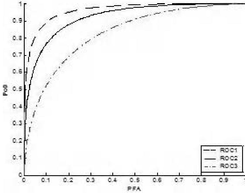
Figure 14.5. Evolution of the Probability of Detection ( PoD ) as a function of the probability of false alarm ( PFA ): Receiver Operating Characteristic ( ROC ) curves for the Probabilities of Crack Existence ( PCE ) under various conditional probabilities P_i
