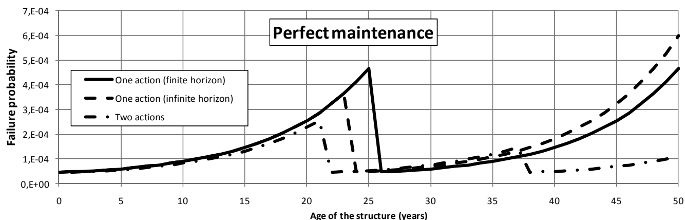
Figure 14.10. Evolution of the failure probability (perfect maintenance)
