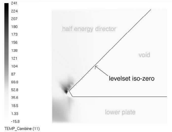
Figure 6 : Temperature field calculated at time 2.3 ms which is equivalent to the 12 th time step.
