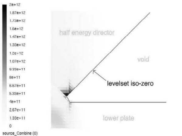
Figure 5 : Source term calculated from the elastic problem for the first time step.
