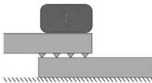
Figure 1 : Ultrasonic welding of two plates
