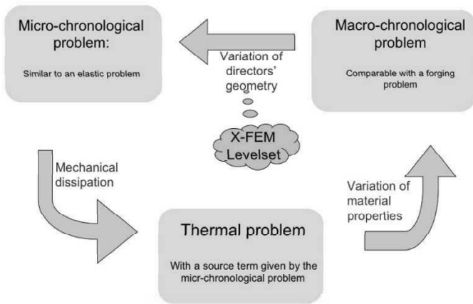
Figure 4 : Solving scheme.
