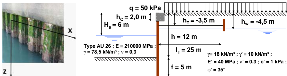
Figure 4. Main geometrical and mechanical characteristics of the quay.
