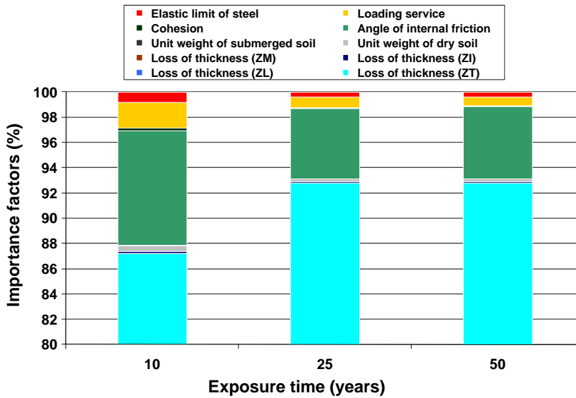
Figure 9. Evolution of importance factors with time (tie-rod zone).
