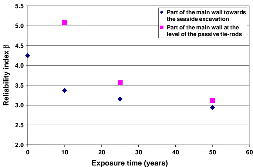
Figure 7. Evolution of the reliability index with time.
