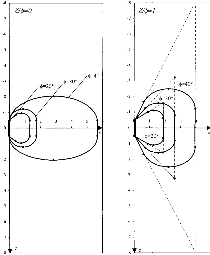
FIG. 10. Traces in Plan View of Mn Mechanism for \phi = 20^\circ, 30^\circ, 40^\circ ; \delta/\phi = 0 and 1 ; and b/h = 1
