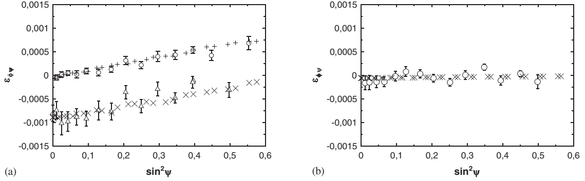
Fig. 1 Intergranular deformations as a function of \sin^2 \psi at room temperature with \phi = 0^\circ for a) – zirconium – \circ \{10\bar{1}4\} and \triangle \{20\bar{2}2\} diffracting plane – experimental result. +, \times : predicted results. b) – titanium – \circ \{30\bar{3}2\} diffracting plane – experimental result. \times : predicted results.
