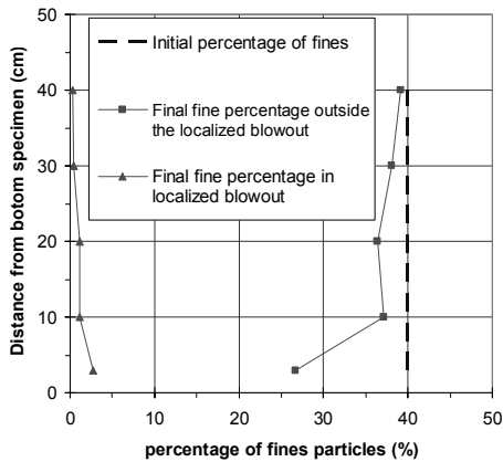
Figure 12. Vertical profiles of fine percentage in specimen
