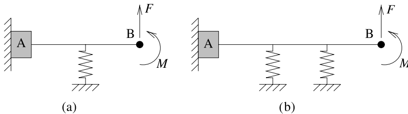
Fig. 3. Features of element A ensure that the vertical displacement and rotation of point B under loading force F and torque M are equal in both cases (a) and (b).
