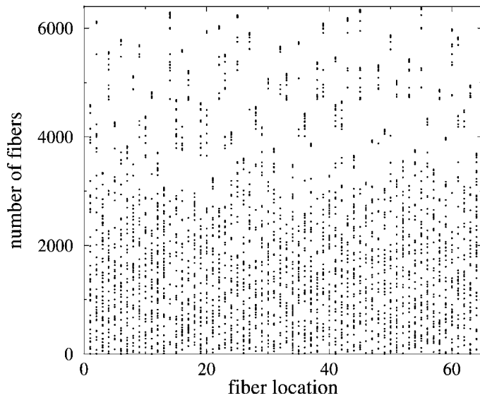
Fig. 11. In the case k < \kappa , the localisation of broken fibers into a bundle could be seen at the end of the loading. In the beginning of the loading (before bifurcation), no localisation occurs.
