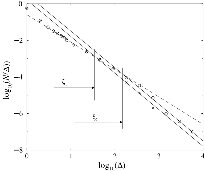
Fig. 5. Avalanche distributions for two elastic bodies stiffnesses. They exhibit the expected two power-laws. The cross-overs (called \xi_1 and \xi_2 ) give the length of the FPZ size.
