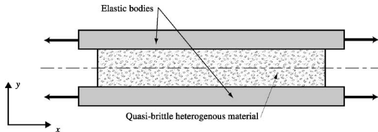
Fig. 6. A scheme of a PIED experimental setup.
