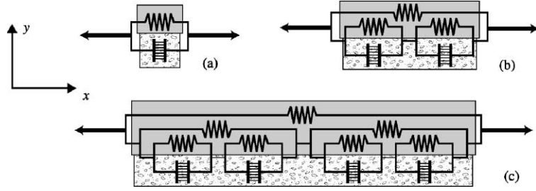
Fig. 7. The hierarchical decomposition for systems of generation 1 (a), 2 (b) and 3 (c).
