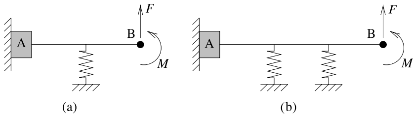
Fig. 3. Features of element A ensure that the vertical displacement and rotation of point B under loading force F and torque M are equal in both cases (a) and (b).
