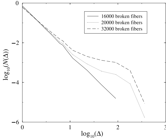
Fig. 12. Evolution of avalanche distribution for a hierarchical model of generation 6 with 1000 fibers per bundle. The distribution is plotted after 16000 broken fibers (before bifurcation), 20000 and 32000 (after bifurcation).
