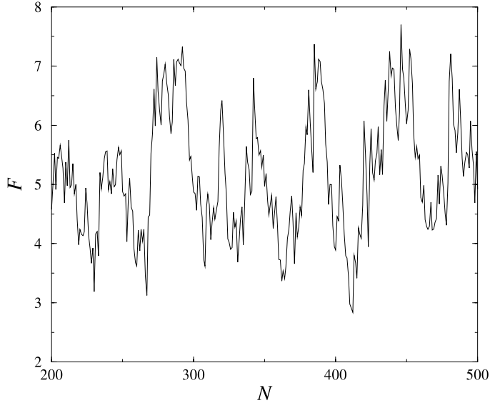
Fig. 2. A part of ZIP model response. x-axis represents the number of broken fibers, y-axis is the value of the global force F .
