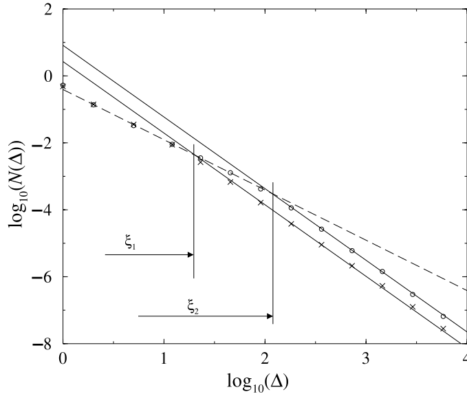
Fig. 4. Avalanche distributions for two beam stiffnesses. They exhibit two power-laws, the first one with an exponent \tau_1 = 1.50 \pm 0.05 (---) and the second one with an exponent \tau_2 = 2.05 \pm 0.10 (—). The cross-over between the two slopes gives the size of the active area ( \xi_1 and \xi_2 on the figure).
