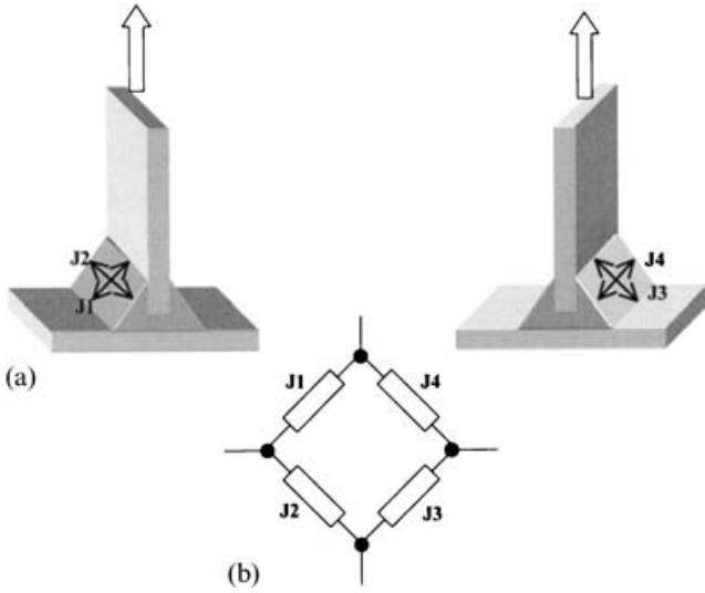
Fig. 5 Tension-compression sensor: (a) gauge positions; (b) wiring diagram. Plane strain assumption: \varepsilon_t = tension strain; \varepsilon_b = bending strain; k = gauge factor; \alpha\Delta t = response to temperature variation; J1 = k*(\varepsilon_t + \varepsilon_b) + \alpha\Delta t ; J3 = k*(\varepsilon_t - \varepsilon_b) + \alpha\Delta t ; J2 = \alpha\Delta t ; J4 = \alpha\Delta t ; R = J1 + J3 - J2 - J4 > R = 2*k*\varepsilon_t
