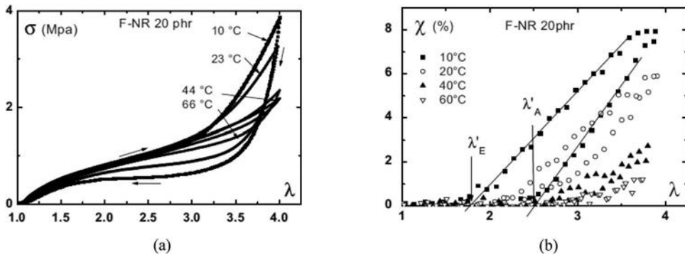
FIG. 18. — Influence of temperature on: (a) stress-strain curve and (b) crystallinity vs stretch ratio for a filled vulcanized NR (20 phr CB, 1.2 phr sulfur). (Reprinted with permission from ref 49. Copyright 2006 Springer.)
