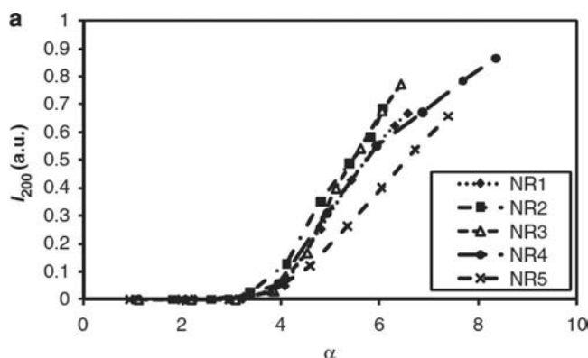
FIG. 15. — Influence of crosslinking on the intensity of (200) spot for vulcanized NR samples: crosslink density is 2.12 , 1.78 , 1.46 , 1.31 , and 1.01 \times 10^4 mol/cm 3 for samples NR1, NR2, NR3, NR4, and NR5, respectively. (Reprinted with permission from ref 15. Copyright 2010 The Society of Polymer Science.)
