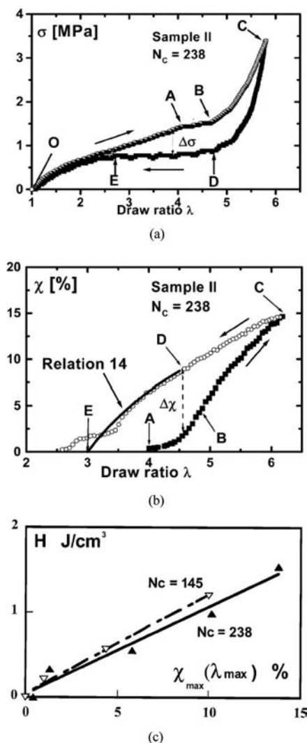
FIG. 12. — Simultaneous evolution of: (a) stress and (b) crystallinity vs stretch ratio, during a tension-retraction cycle (strain rate \sim 5 \times 10^{-4} \text{ s}^{-1} ) at 22 °C for a vulcanized NR (1.2 phr sulfur). (c) Evolution of the mechanical hysteresis vs the maximum crystallinity measured at the maximum stretch ratio for different samples of two vulcanized NR containing: 1.2 phr sulfur (black triangles), 2 phr sulfur (white triangles). (Reprinted from ref 61. Copyright 2003 American Chemical Society.)
