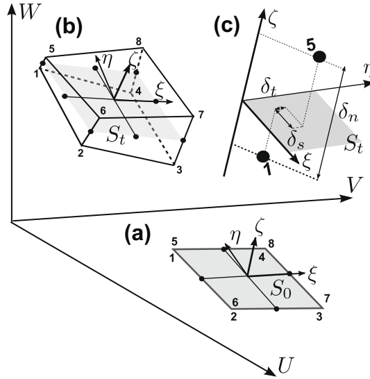
Fig. 5. An interface element in its initial configuration (a) and its deformed configuration (b), and characterization of the separation of two nodes in the deformed configuration (c).
