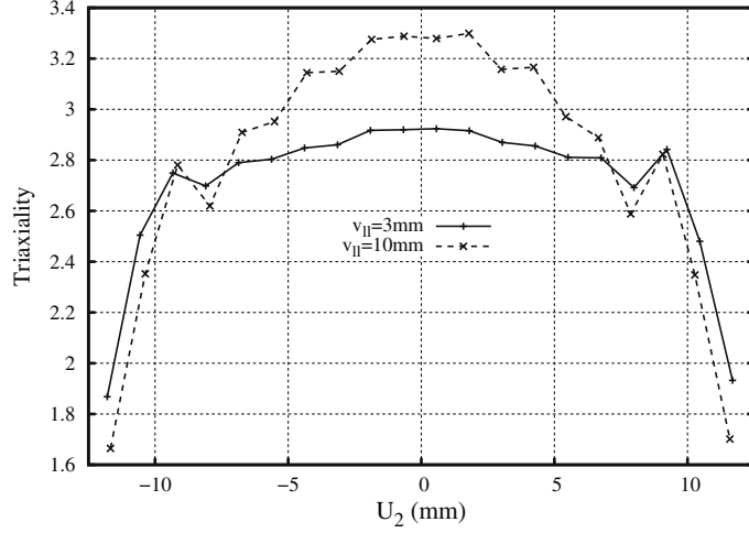
Fig. 14. Maximum triaxiality along the front.
