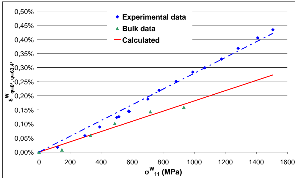
Figure 3: Strain deduced from the shift of the W(310) diffraction peak measurements \blacklozenge as a function of estimated applied stress increment (the first loaded state being chosen as the reference state) in W layers along the loading axis, for \psi = 63.4^\circ and \varphi = 0^\circ , for the thinnest W layer thickness. ( \lambda_{XR} = 0.127 nm). The dotted line represents the linear regression obtained from experimental data while the continuous line is calculated from equations (2) and (3) considering bulk elastic constants. The straight red line fits well the elastic strain \blacktriangle measured on a 200-nm-thick tungsten layer (performed with similar deposition conditions) following W(211) diffracting plane ( \psi = 61.9^\circ and \varphi = 0^\circ ).
