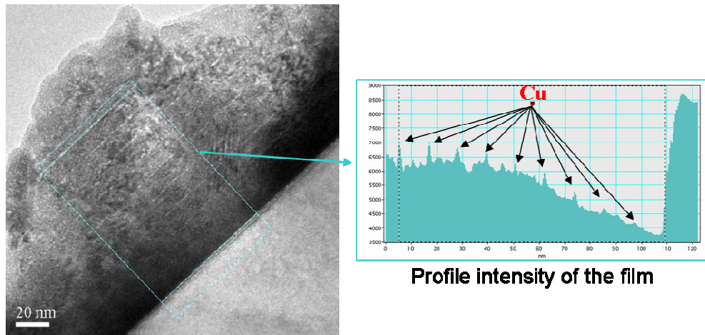
Figure 1: TEM Bright Field realized on W/Cu 10.8/0.2 showing the thin film stratification and suggesting copper layer discontinuities (confirmed by GISAXS).
