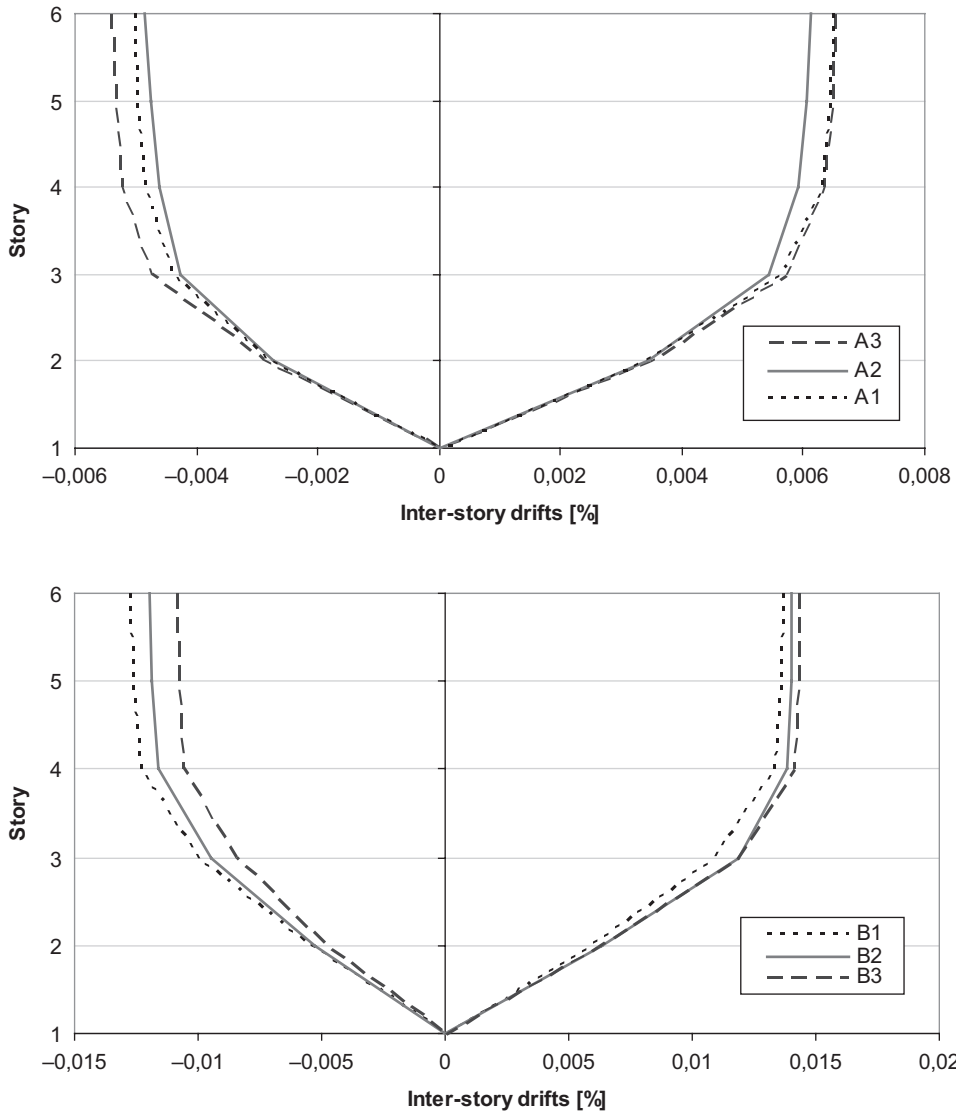
FIGURE 28 Simplified model: 3D loading, inter-story drifts (XG wall).
