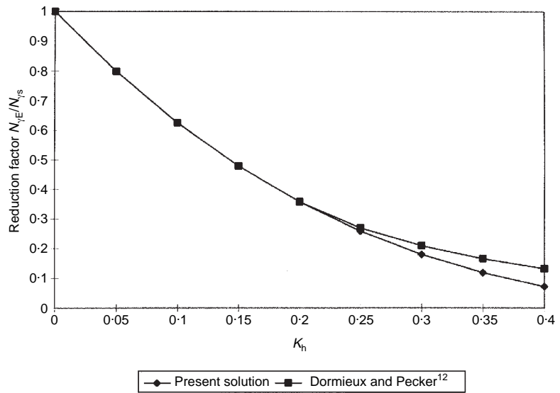
Fig. 4. Comparison of the present solution and that of Dormieux and Pecker 12 for the M1 mechanism ( \phi = 30^\circ )
