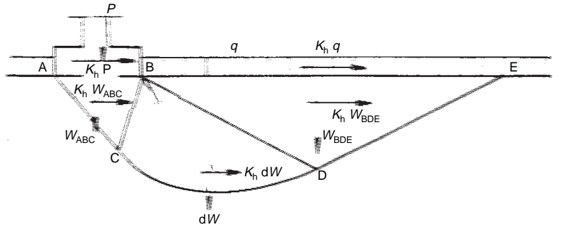
Fig. 2. Free body diagram for the M1 mechanism
