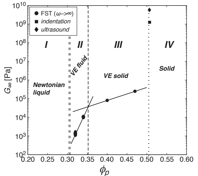
Fig. 10 High frequency elastic modulus, G_\infty , as a function of particle volume fraction. Symbols indicate the methods employed. The symbol size represents the measurement uncertainty. For the solid samples, G_\infty is calculated from the Young's Modulus through the relationship G_\infty = E/2(1+\nu) (Mezger, 2002). Four different rheological regimes can be identified as \phi_p increases.
