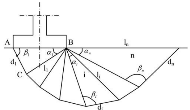
Fig. 3. Failure mechanism M2 for seismic bearing capacity analysis
