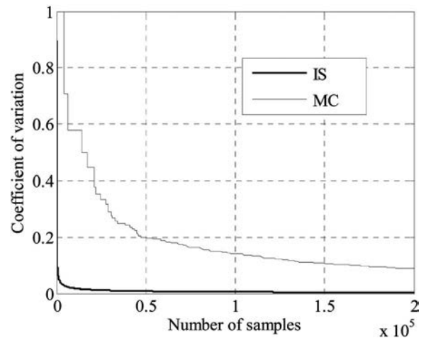
Fig. 7. Coefficient of variation of the failure probability versus the number of samples
