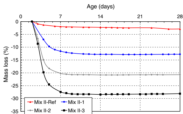
Fig. 11. Mass loss of the PUR-foam concrete mixtures ( T = 20 \pm 2 \text{ }^\circ\text{C} ; \text{RH} = 50 \pm 5\% ).
