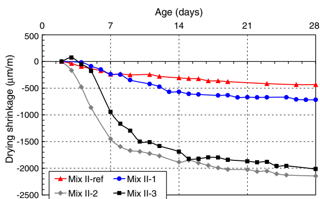
Fig. 12. Drying shrinkage of the PUR-foam concrete mixtures ( T = 20 \pm 2 \text{ }^\circ\text{C} ; \text{RH} = 50 \pm 5\% ).
