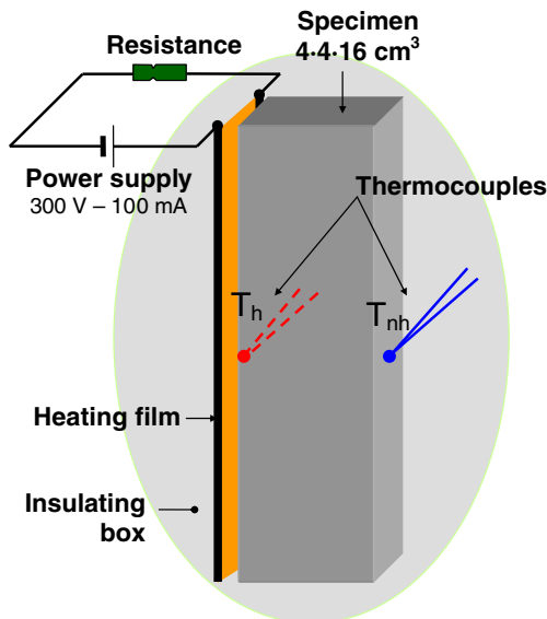
Fig. 5. Diagram of the experimental device used for the determination of the thermophysical properties of the concrete mixtures.
