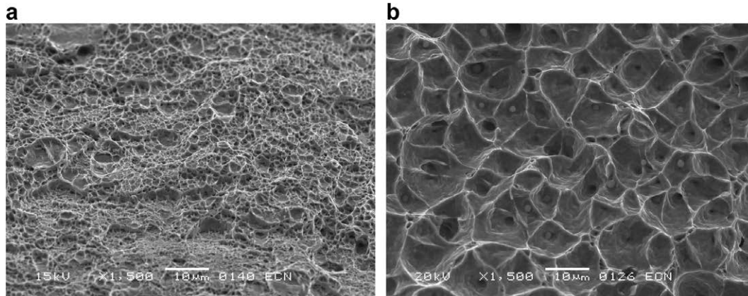
Fig. 11. Fracture topography in TIG welded zone (a) and A-TIG welded zone (b) observed under SEM.
