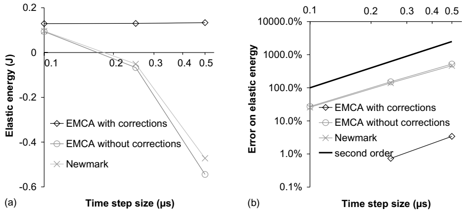
Fig. 11. Final energy (after 80 \mu\text{s} ) for the Taylor bar: (a) elastic energy, (b) error on elastic energy.
