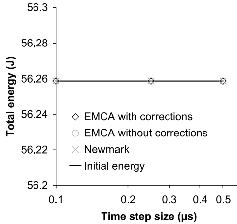
Fig. 12. Final total energy (after 80 \mu\text{s} ) for the Taylor bar.
