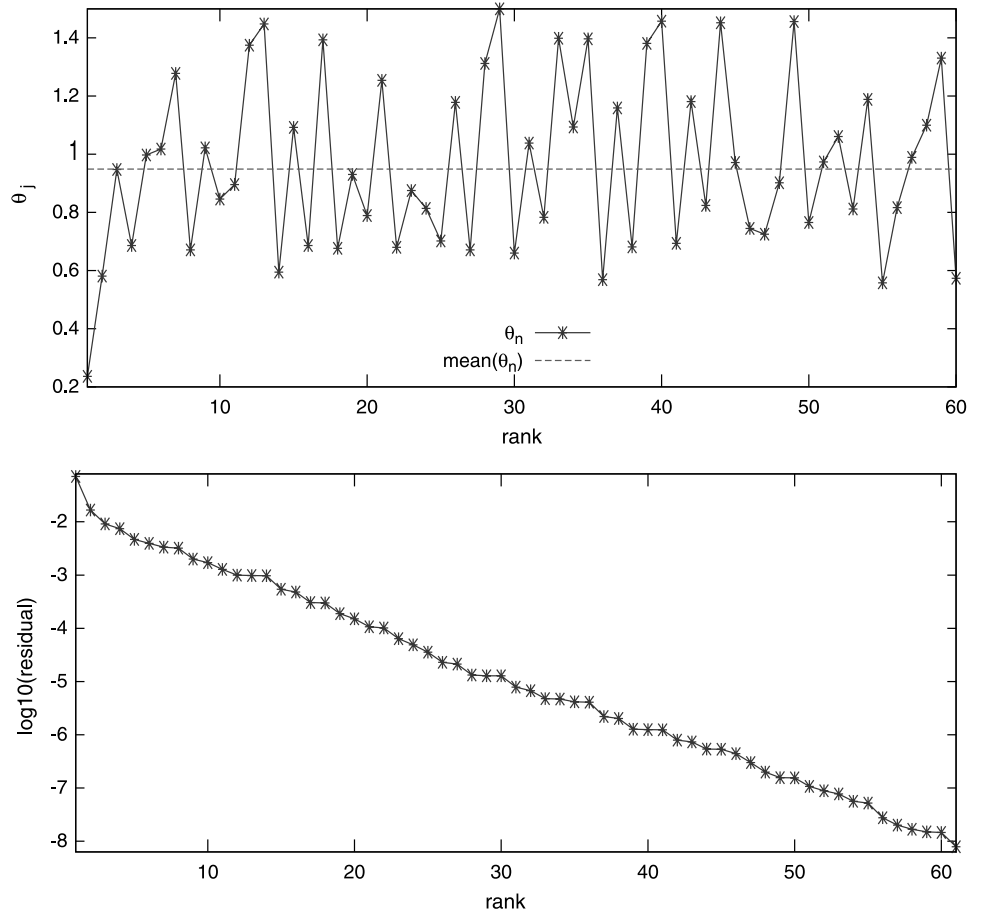
Fig. 2 The sequences \{\theta_j\}_{j=1}^{62} , and \{\log_{10} \|\mathbf{r}^j\|_2\}_{j=0}^{62} when we take as a choice of A a 20 \times 20 random matrix
