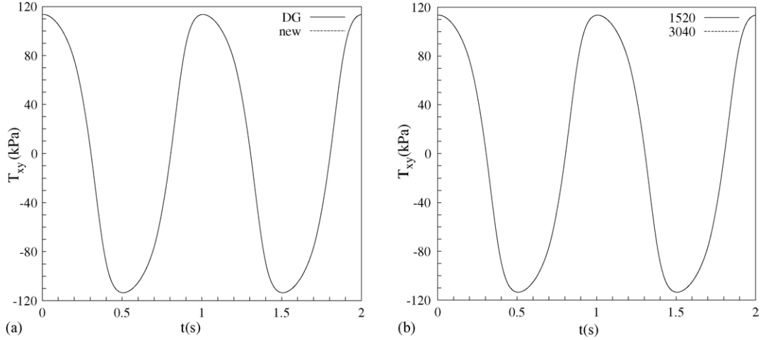
Fig. 4. Validation of the numerical technique. Comparison of: (a) new method with the DG method of [9] and (b) various \tau discretizations.
