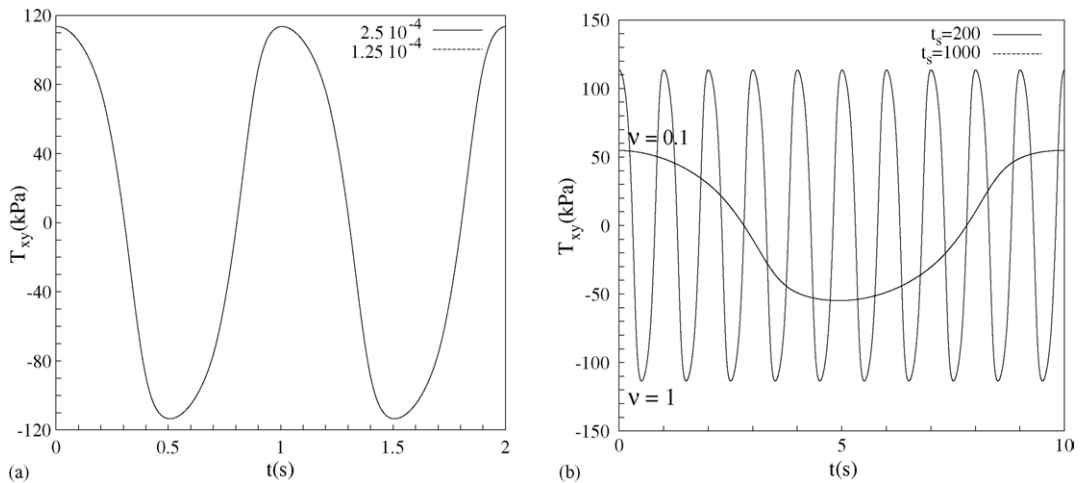
Fig. 5. Validation of sufficiently small time step (a) and sufficiently large t_s (b).
