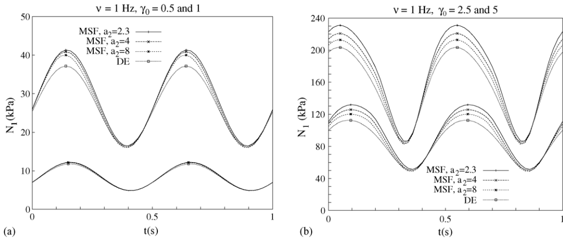
Fig. 11. Comparison of N_1 predictions for the MSF model using values of a_2 as indicated in the legends and the Doi-Edwards model.
