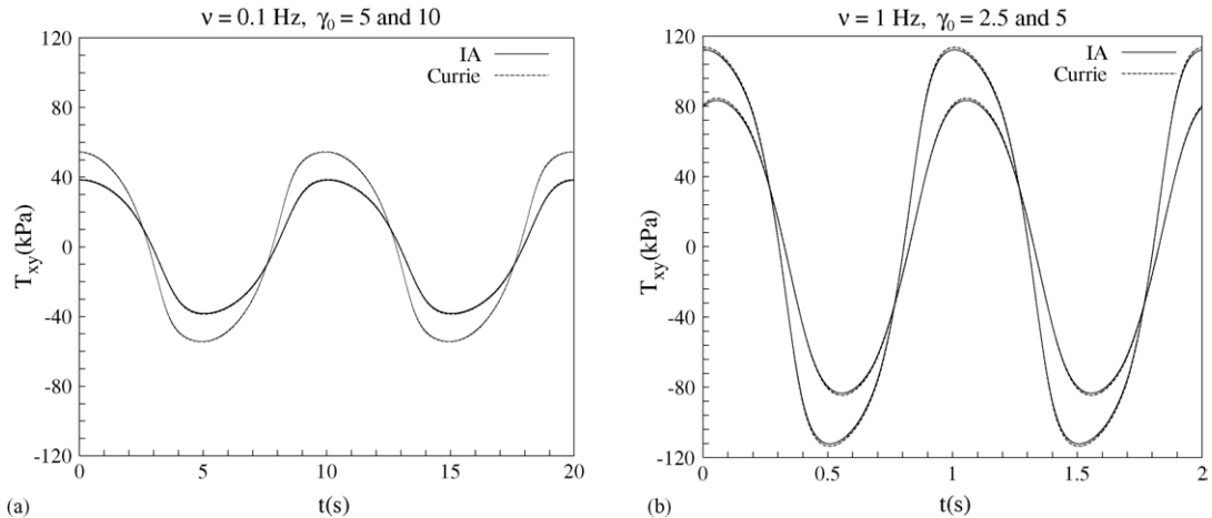
Fig. 6. Comparison of the steady periodic shear stress prediction of the MSF model using the Currie and independent alignment approximation at amplitudes \gamma_0 indicated in the figures: (a) \nu = 0.1 Hz and (b) \nu = 1 Hz.
