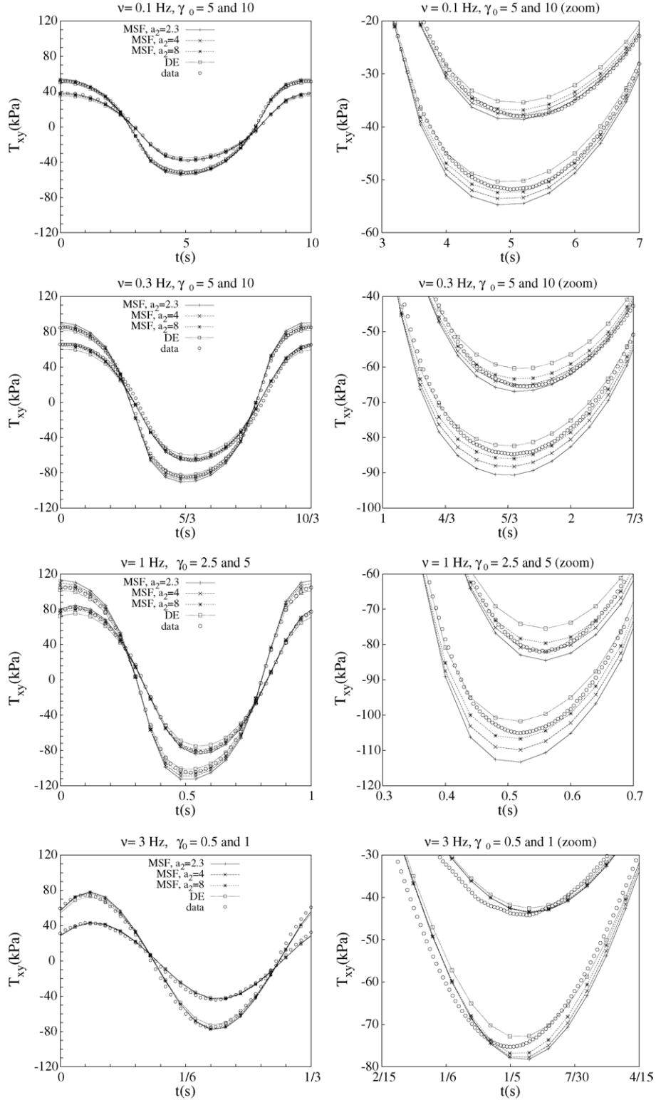
Fig. 9. Comparison of MSF model using values of a_2 as in the legends and Doi–Edwards model with periodic shear stress data for Finathene melt [8]. Left column: one period; right column: zoom around minimum.
