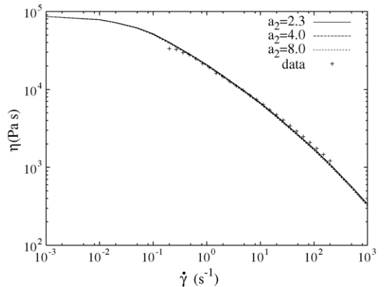
Fig. 1. Steady shear viscosity of the Finathene melt: experimental data of [8] and model predictions of the MSF model using various values of a_2 ( a_1 = 0.02 ).
