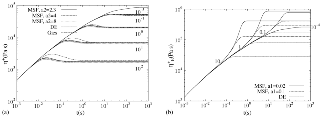
Fig. 3. Transient viscosity of MSF model for various parameter settings. The Doi–Edwards and Giesekus model are included for comparison. Deformation rates ( \text{s}^{-1} ) are indicated in the figures. Start up of: (a) shear for a_1 = 0.02 and values of a_2 indicated in the legend and (b) uniaxial elongation for values of a_1 indicated in the legend ( a_2 irrelevant).
