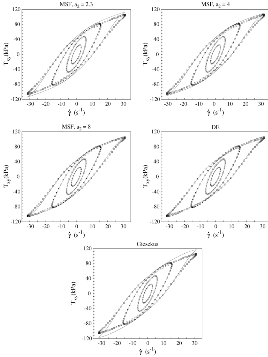
Fig. 10. Lissajous plots for \nu = 1 Hz for Finathene data of [8] and model predictions. Strain amplitudes \gamma_0 are 0.5, 1, 2.5, and 5 (from innermost to outermost loops).
