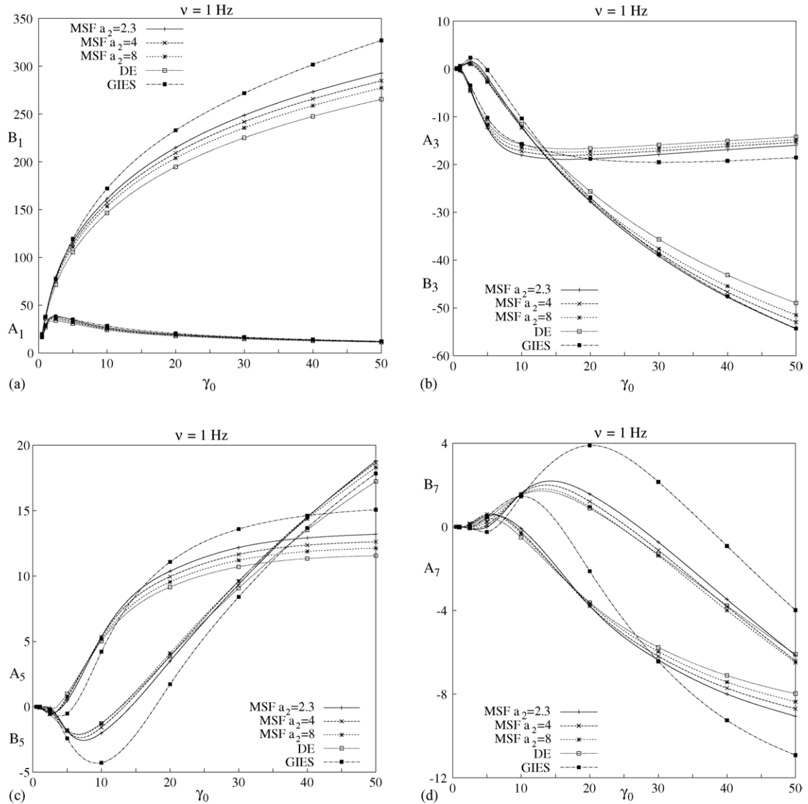
Fig. 12. (a-d) Amplitudes A_n and B_n of the odd harmonics (kPa) outside the experimental window for MSF model using values of a_2 as in the legends. The Doi-Edwards and Giesekus model are included for comparison.
