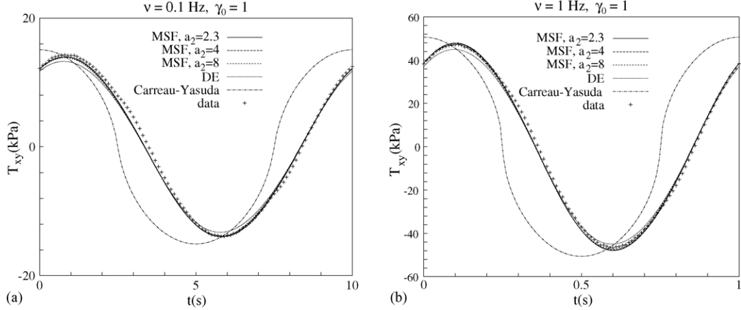
Fig. 8. Periodic shear stress at moderate shear rates predicted by the viscous and viscoelastic models together with the Finathene data. Frequencies and strains indicated in the figures.
