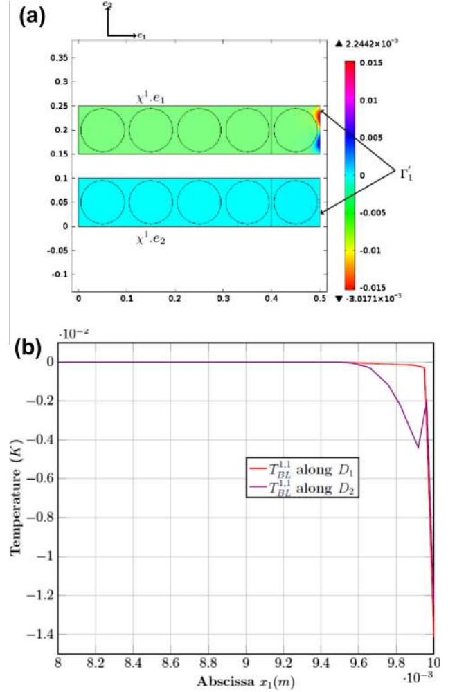
Fig. 15. Numerical solutions/ 15a: \chi_i^1(\mathbf{y}) , i = 1, 2 computed on \tilde{G}_1 , truncated at d_1 = 0.5 mm and/15b: T_{BL}^{1,1} along two lines cut (see Fig. 10) on \tilde{G}_1 , truncated at d_1 = 2 mm.
