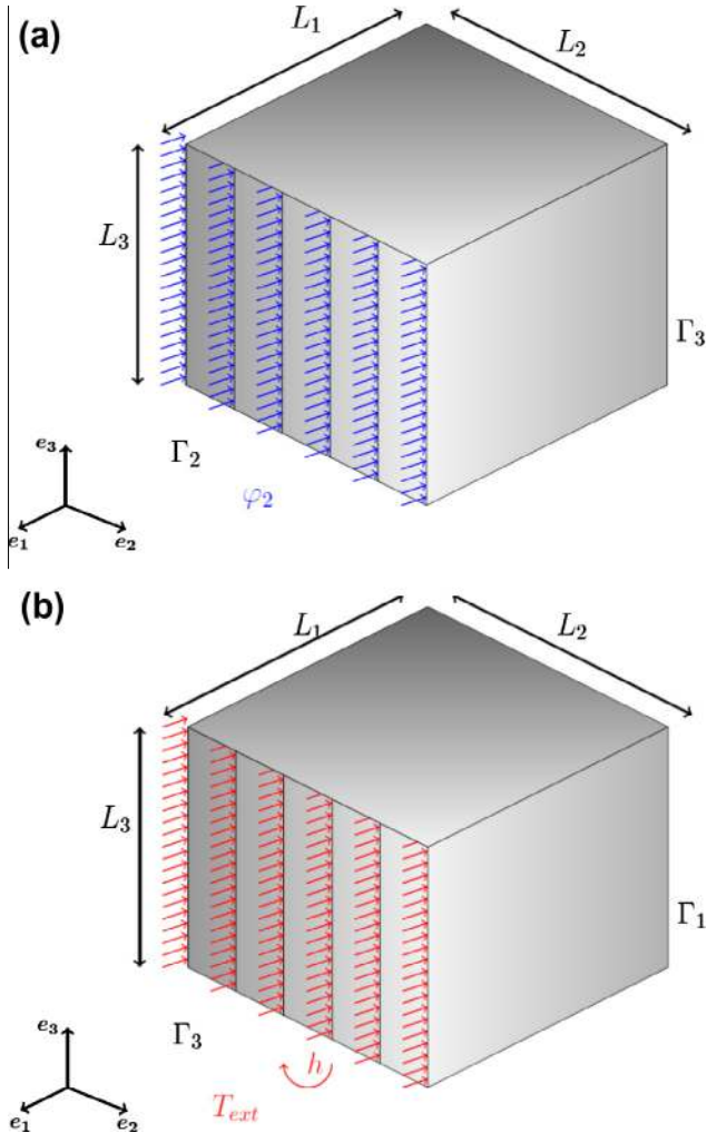
Fig. 2. The 3-D spatial domain \Omega and its boundary conditions: (a) – Neumann & Dirichlet boundary conditions; (b) – Fourier and Dirichlet boundary conditions.
