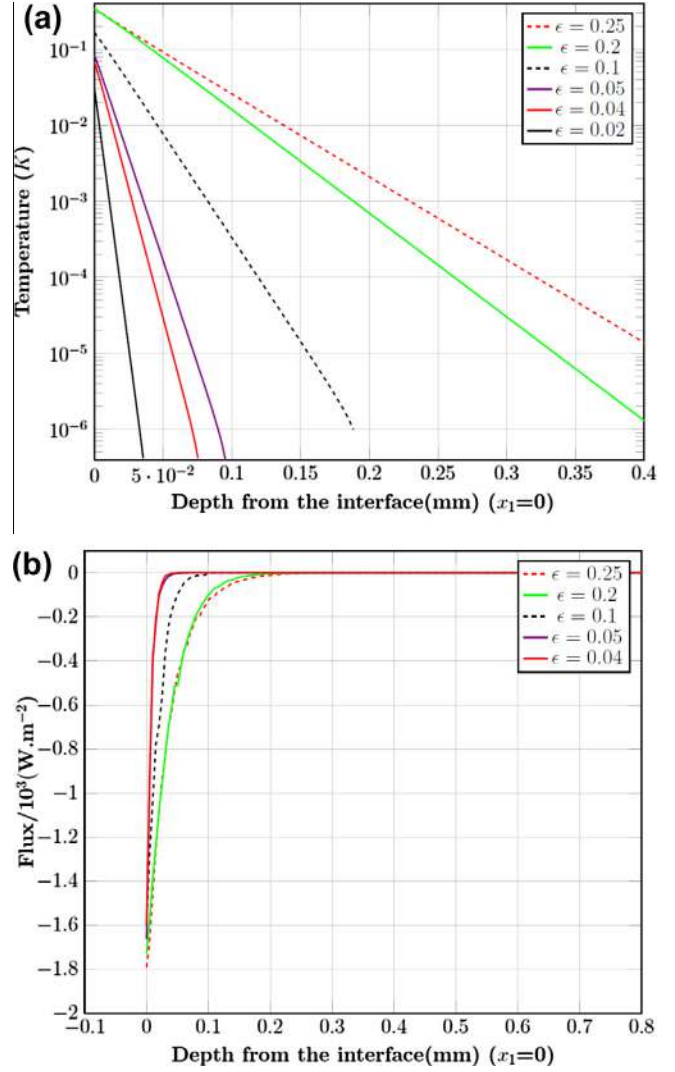
Fig. 6. Influence of the scale ratio \epsilon on the correcting terms T_{BL}^{1,2} and \phi_{BL}^0 \cdot e_1 , versus x_1 , computed on the sub-domain \tilde{G}_2 , truncated at d_2 = 0.8 mm/ (a): temperature T_{BL}^{1,2} / (b): Heat flux density \phi_{BL}^0 \cdot e_1 (in the insulating layer, i.e. along the red line drawn on Fig. 4b). (For interpretation of the references to color in this figure legend, the reader is referred to the web version of this article.)
