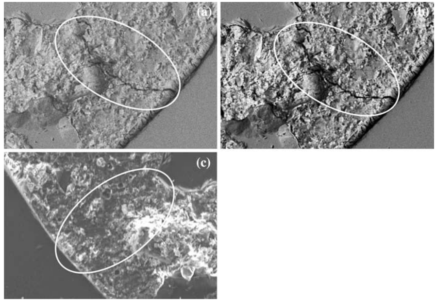
Fig. 3 BSE of mortar A in low- and high-vacuum mode (a, b) and SEI of the replica (c), (200 days, 600×)
