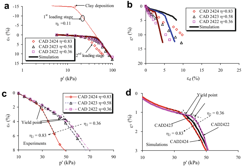
Fig. 14. Model prediction for tests with stress ratio \eta bigger than that of previous consolidation stage \eta_1 .
