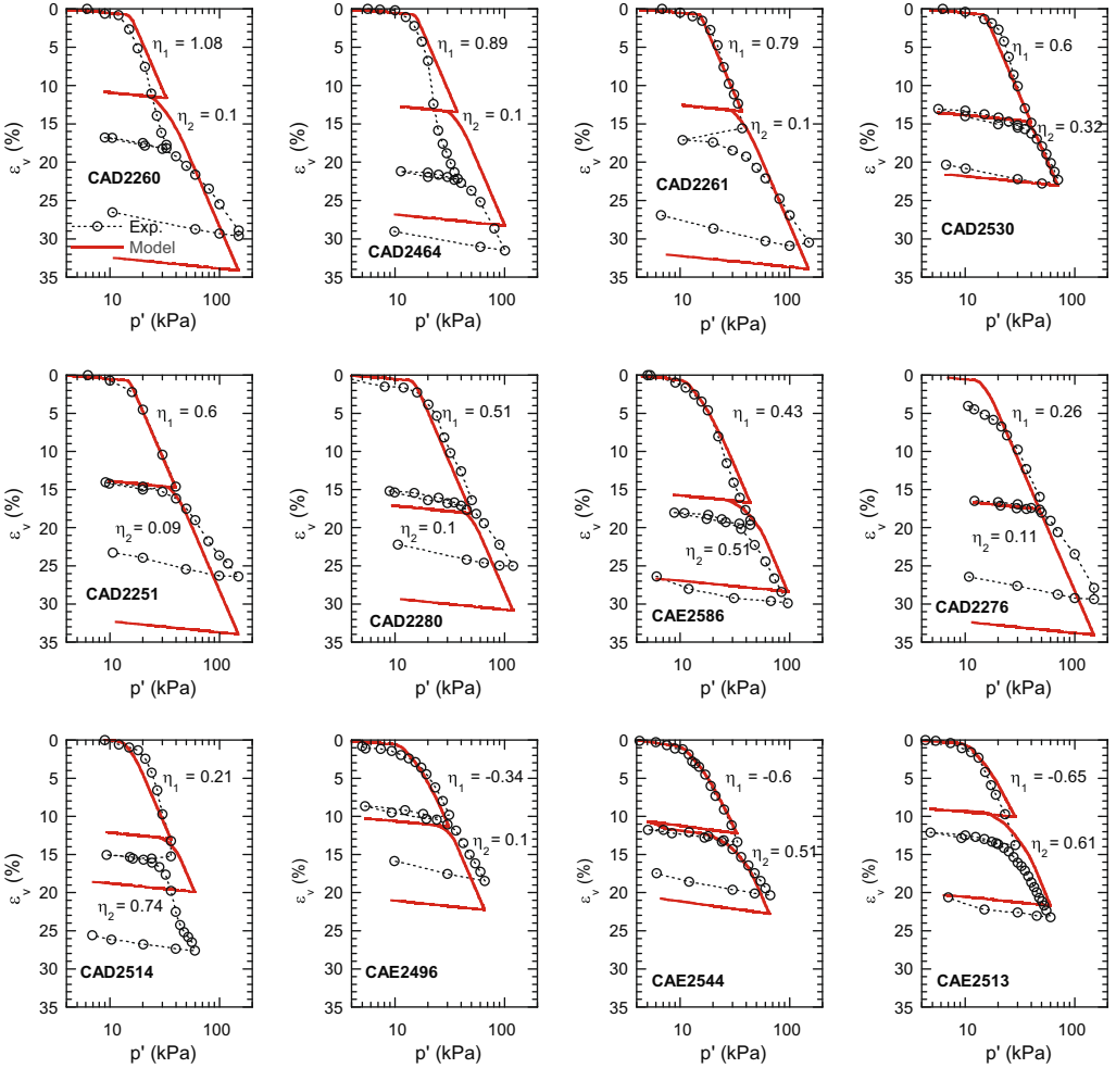
Fig. 17. Model predictions on drained tests Series A.
