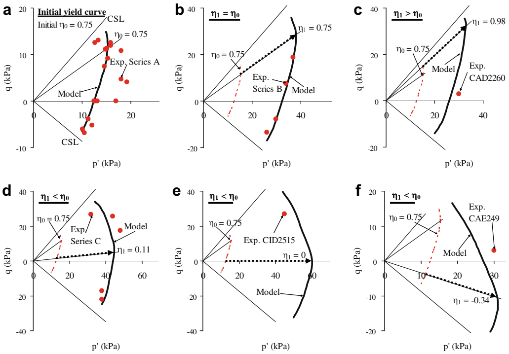
Fig. 19. Initial apparent yield curve and apparent yield curves for different consolidation history.
