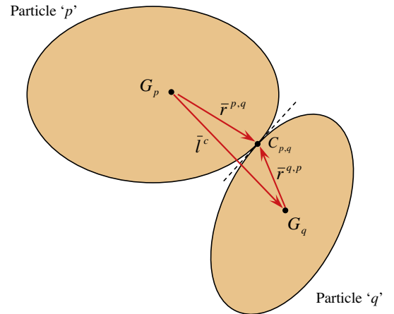
Fig. 1. Particles in contact. Geometrical description.
