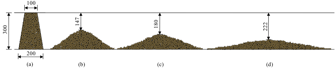
Fig. 2. (Color online.) Slump tests: (a) initial sample, (b) \mu = 0.5 , (c) \mu = 0.3 , (d) \mu = 0.1 .
