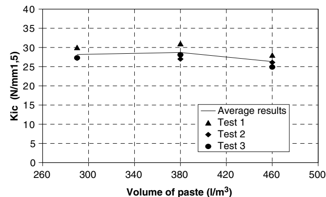
Fig. 20. K_{ic} vs. volume of paste.
