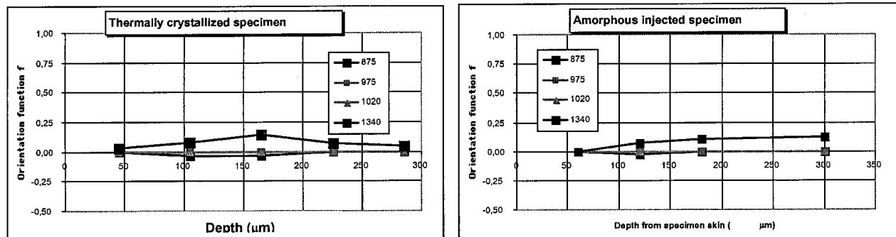
Figure 15: Macromolecular orientation in thermally crystallized PET specimen (left) and non stretched amorphous specimen (right)
