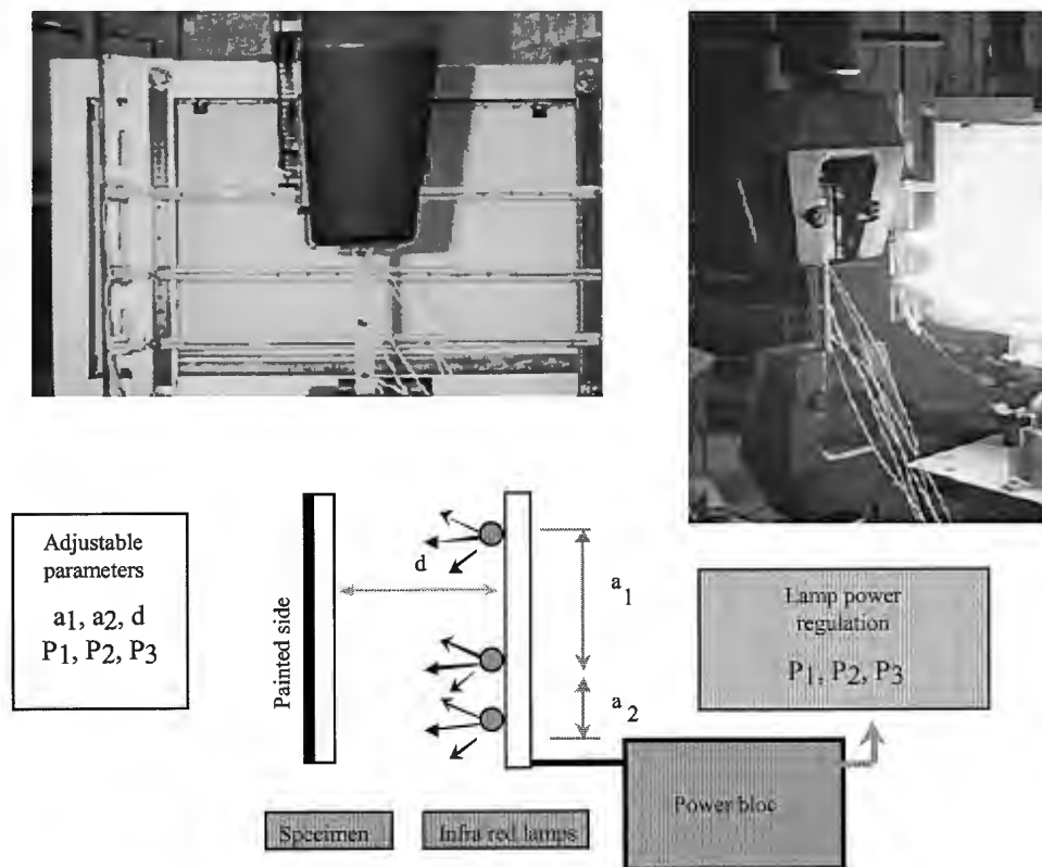
Figure 1: Infra red heating apparatus
