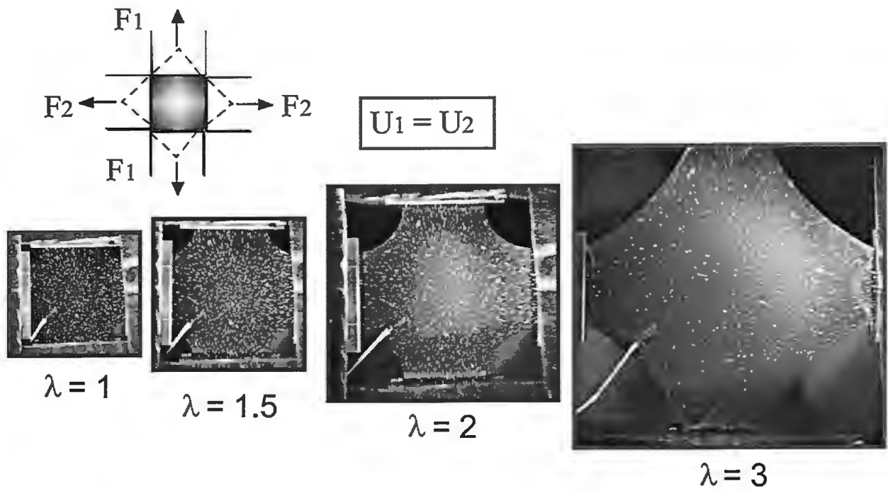
Figure 7: Typical equibiaxial elongation test
