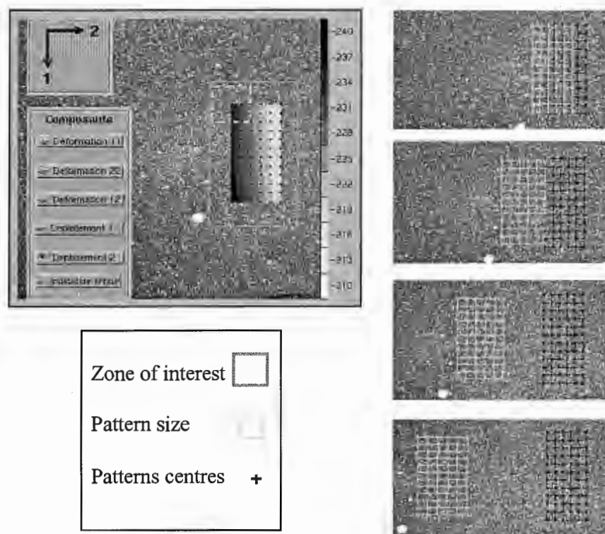
Figure 2: Digital image intercorrelation technique used to measure displacement field (typical uniaxial result)
