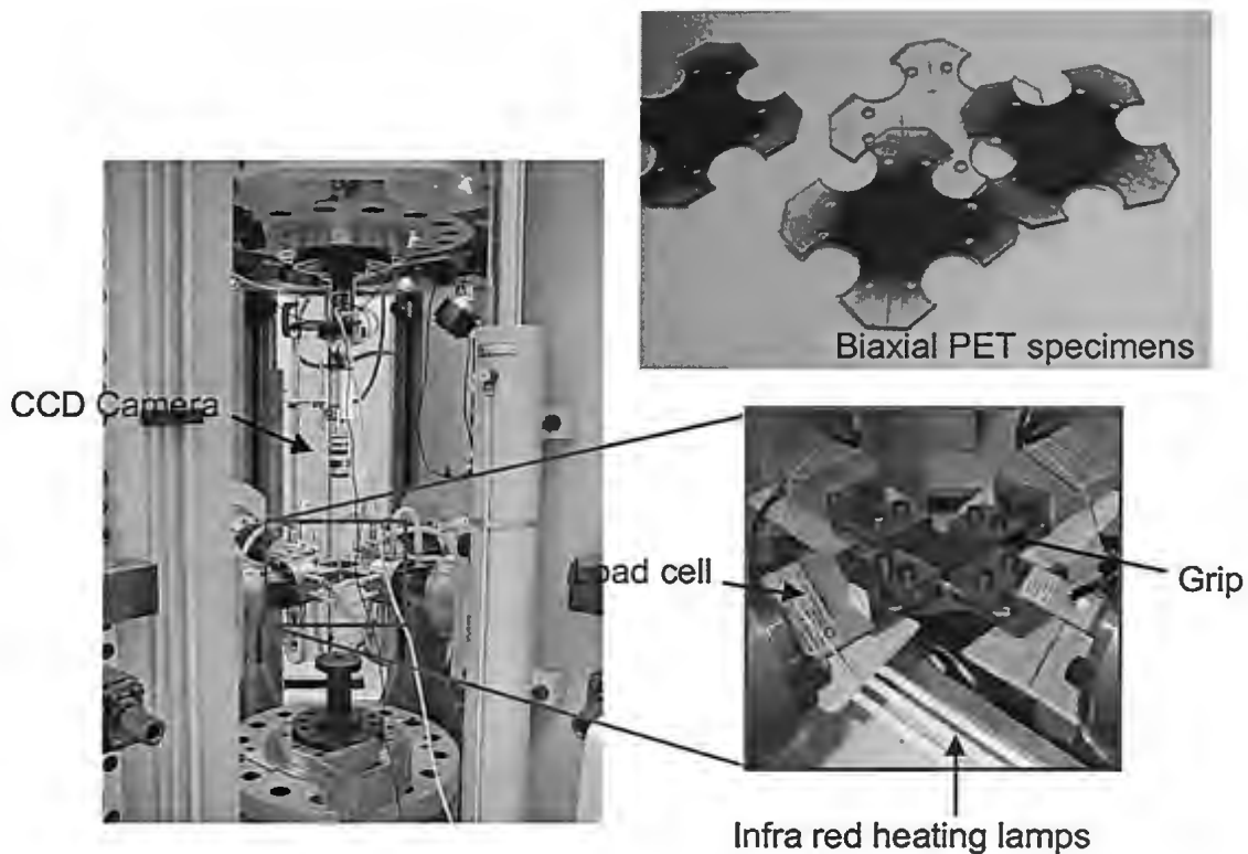
Figure 6: Biaxial testing apparatus, triaxial testing machine Astree, biaxial specimens, IR heating apparatus
