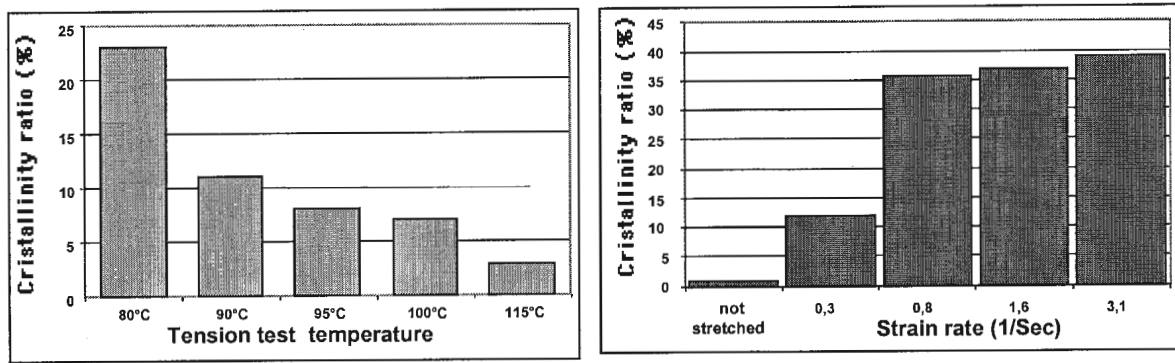
Figure 16: (left) Influence of thermal conditions on induced crystallization for a given tension test elongation speed (8 mm/s) (right) Influence of strain rate conditions on induced crystallization for a given test temperature (90°C)
