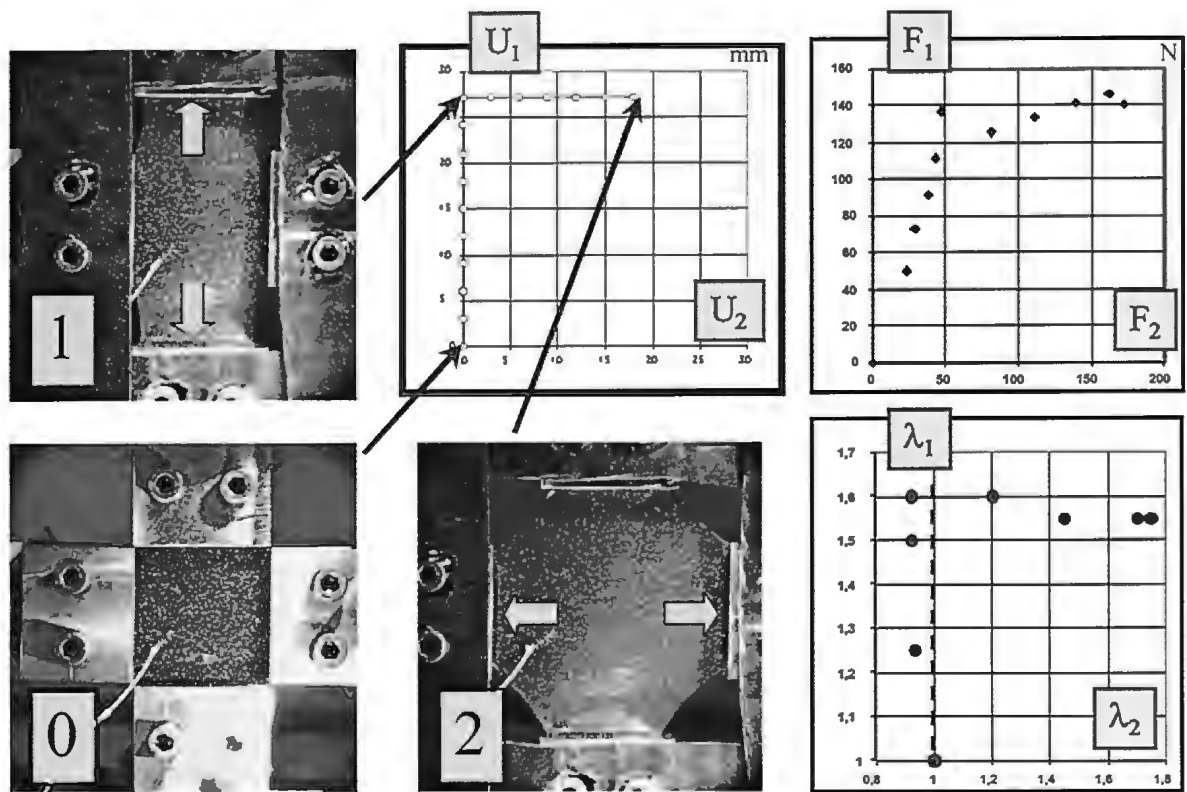
Figure 7: Typical equibiaxial elongation test
