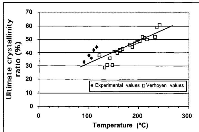
Figure 13: Ultimate crystallinity ratio dependence on temperature
