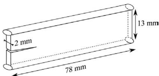
Figure 2 Pure shear specimen.
