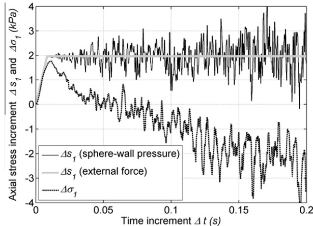
Fig. 7. Time versus the stress increments resulting from the application of \Delta s_1 = 2 \text{ kPa} from the state M_A defined in Fig. 6.
