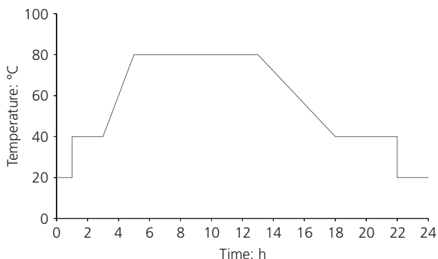
Figure 1. Temperature cycle imposed on the heat-cured mortars
