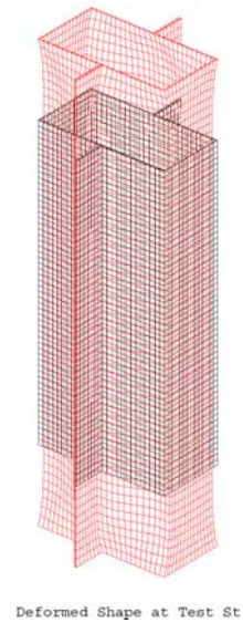
Figure 6 : RVE ECA-R deformed shapes under loading conditions ( E_{11} and E_{33} ), and E_{33}
