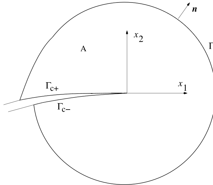
Fig. 23. Notations for the J -integral.
