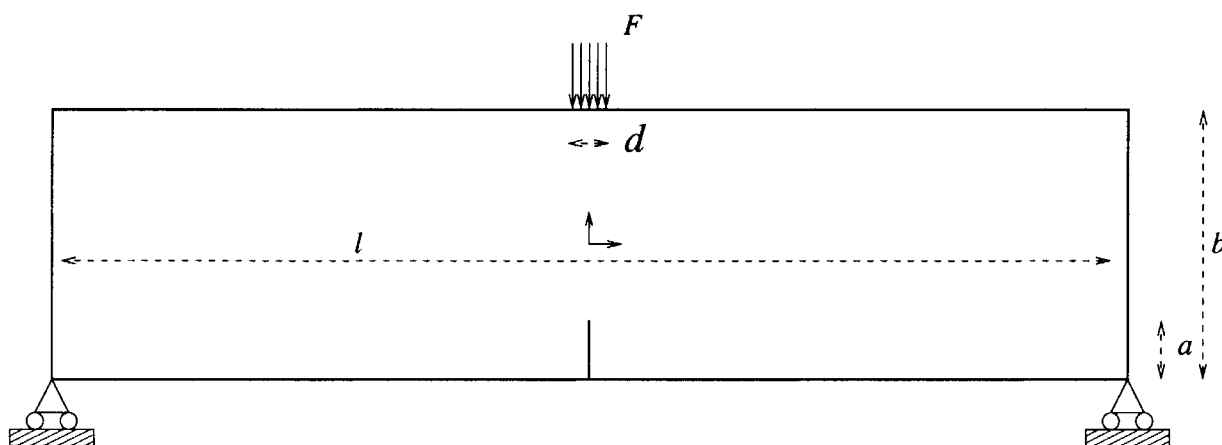
Fig. 8. A three-point bending specimen.
