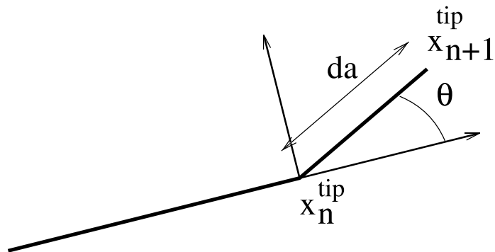
Fig. 5. Notations for a step of growth of the cohesive crack.
