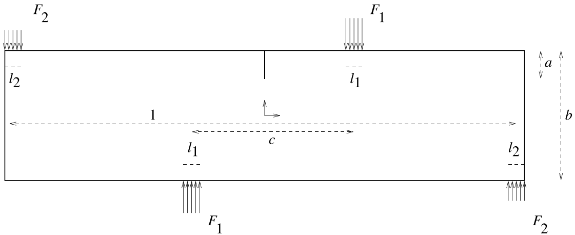
Fig. 17. A four-point shear specimen.
