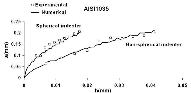
Fig. 6. Comparison between experimental and numerical a(h) curves for AISI 1035.
