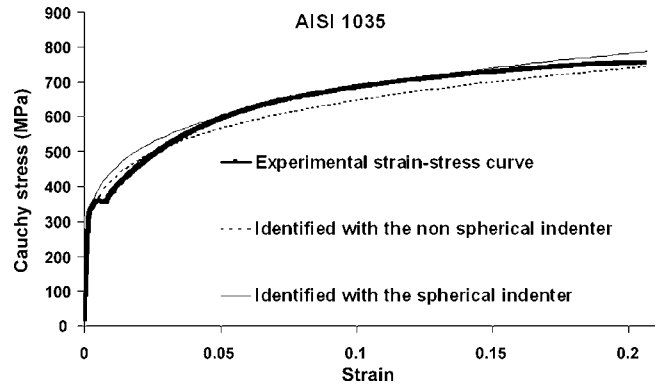
Fig. 10. Determination of stress–strain curve for AISI 1035.
