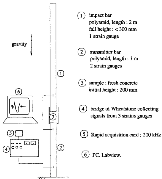
Figure 1 – Experimental device.
