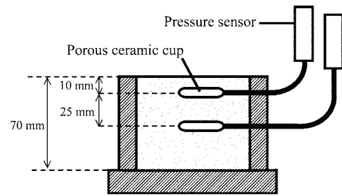
Fig. 3—Schematic section view of capillary pressure measurement.
