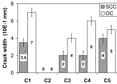
Fig. 19—Maximum crack width of all SCC and OC pairs.
