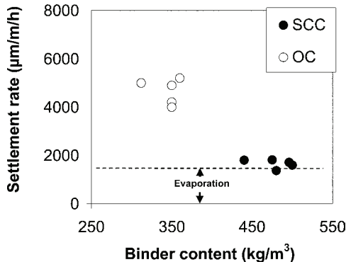
Fig. 13—Initial settlement rate versus powder content of SCC and OC mixtures for no-wind condition.
