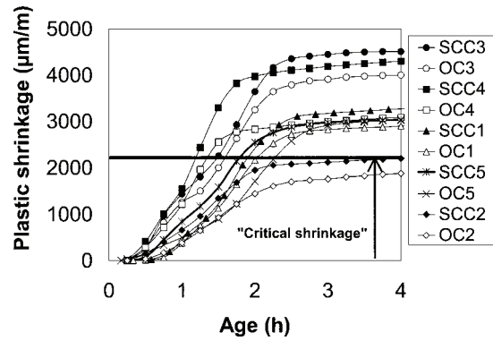
Fig. 16—Plastic shrinkage of SCC and OC mixtures in wind conditions ("critical shrinkage" indicates approximate shrinkage value beyond which specimen cracks).
