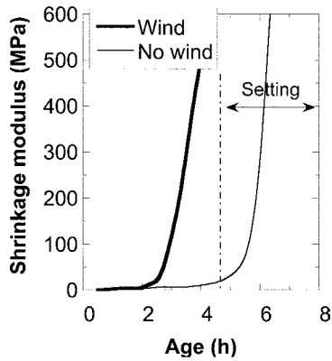
Fig. 11—Shrinkage modulus for both no-wind and wind conditions (Mixture SCC3).
