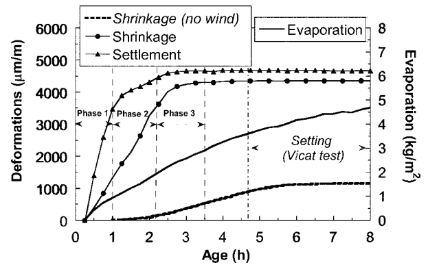
Fig. 9—Plastic shrinkage, settlement, and evaporation for wind condition and plastic shrinkage for no-wind condition (Mixture SCC3).
