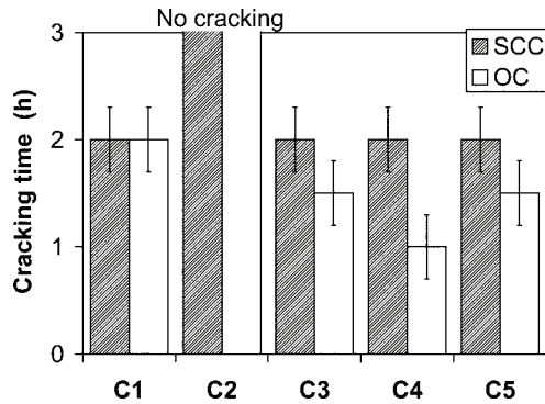
Fig. 20—Cracking time for all SCC and OC pairs.
