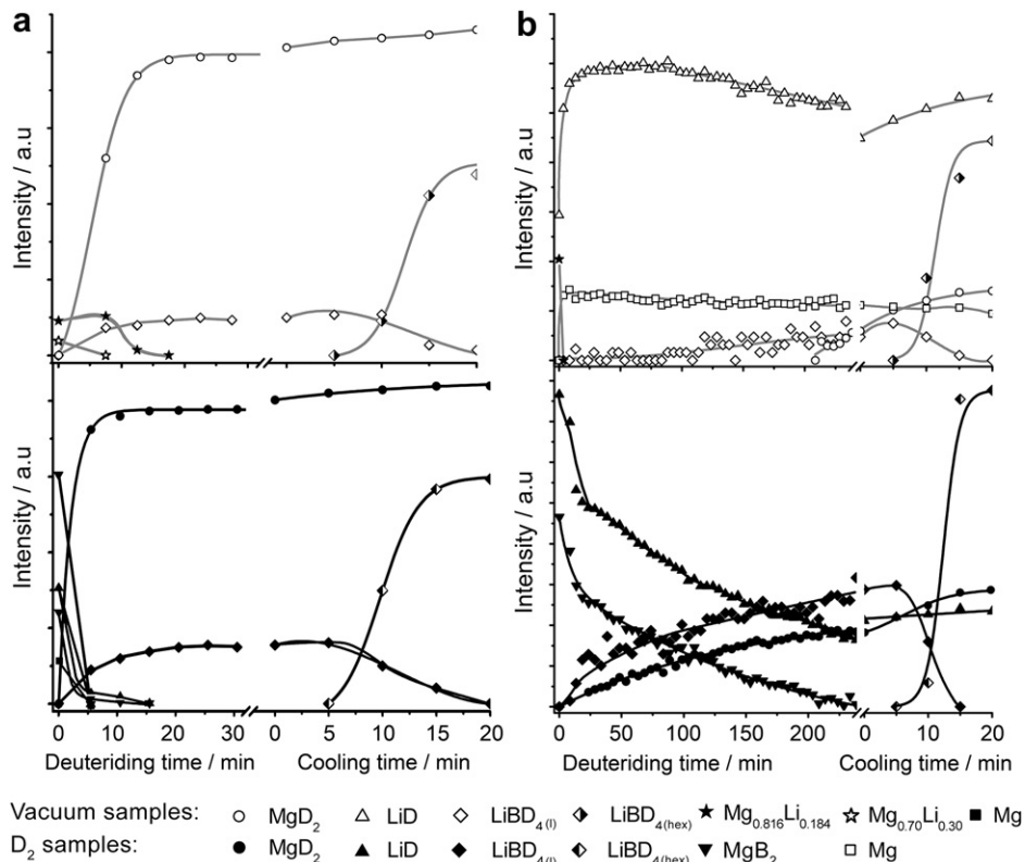
Fig. 4 – Peak intensities during deuteriding at 400^\circ\text{C} and cooling under 100 bar \text{D}_2 pressure. (a) 0.3:1 samples decomposed under vacuum (top) and deuterium (bottom), (b) 2:1 samples decomposed under vacuum (top) and deuterium (bottom).
